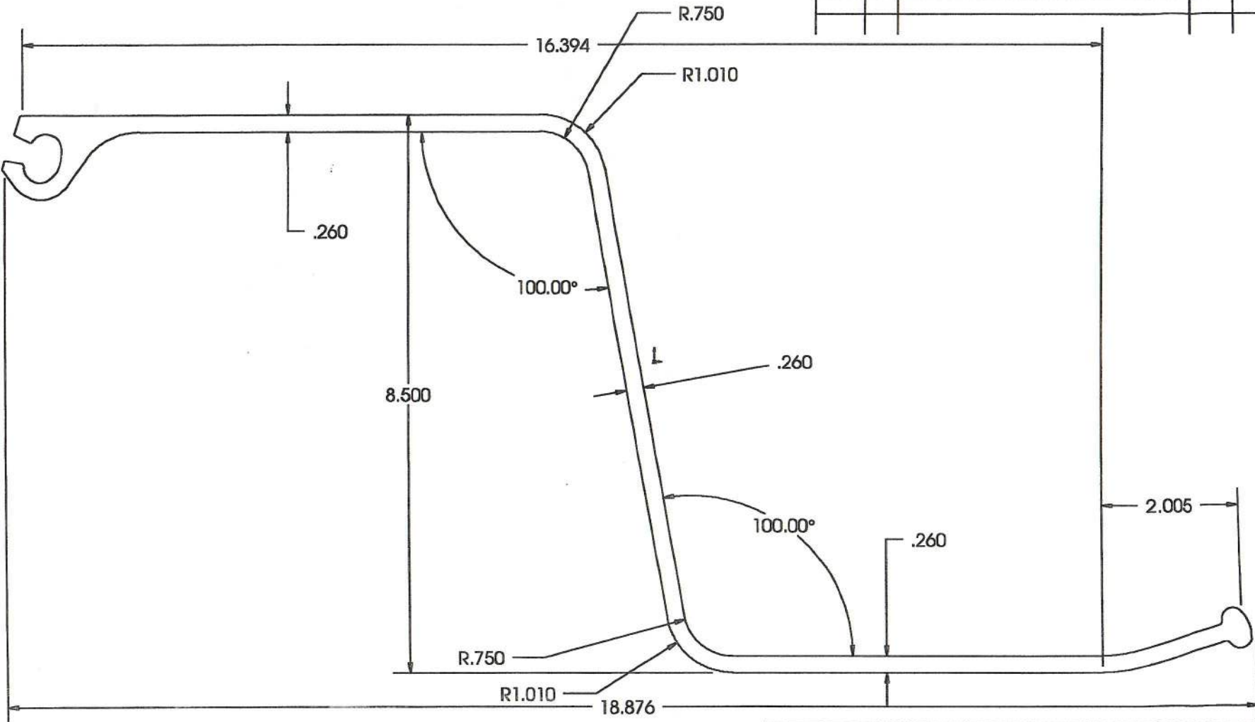
SuperWall Fiberglass Sheetpile 8.5" profile
