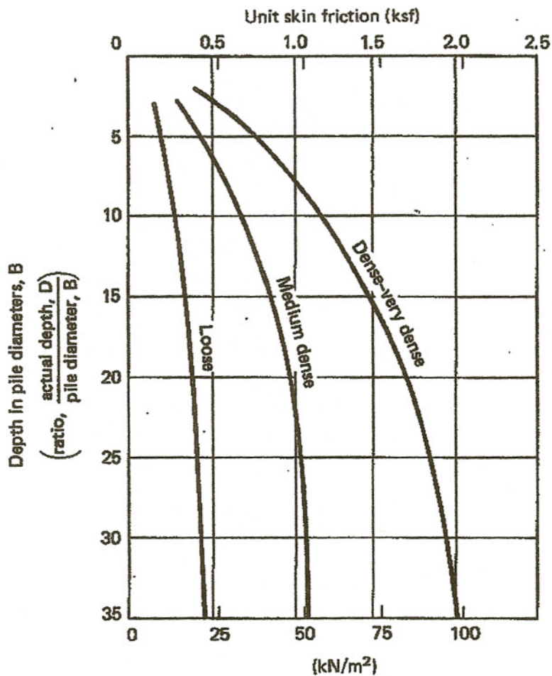
Figure 14-23 Range of values: Skin friction versus depth for straight-sided piles driven in sand. (After Coyle and Castello [51])
